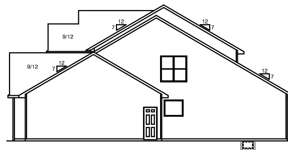
RIGHT ELEVATION 1/2 SCALE
