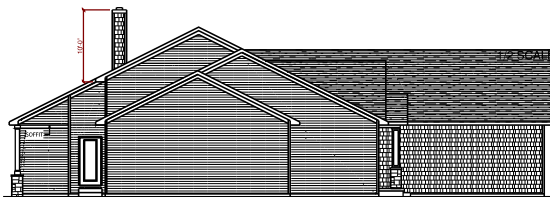
LEFT ELEVATION 1/2 SCALE
