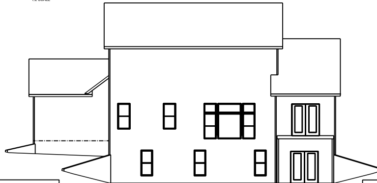
REAR ELEVATION 1/2 SCALE
