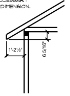
TRUSS DETAIL 1/2" = 1'-0"
