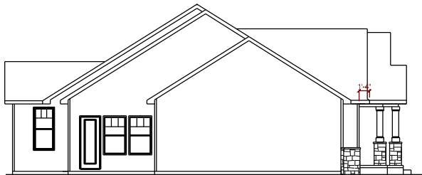
LEFT ELEVATION
