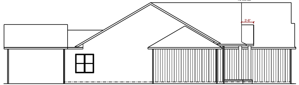
LEFT ELEVATION 1/2 SCALE
