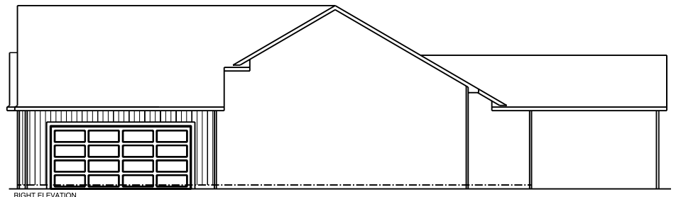
RIGHT ELEVATION 1/2 SCALE
