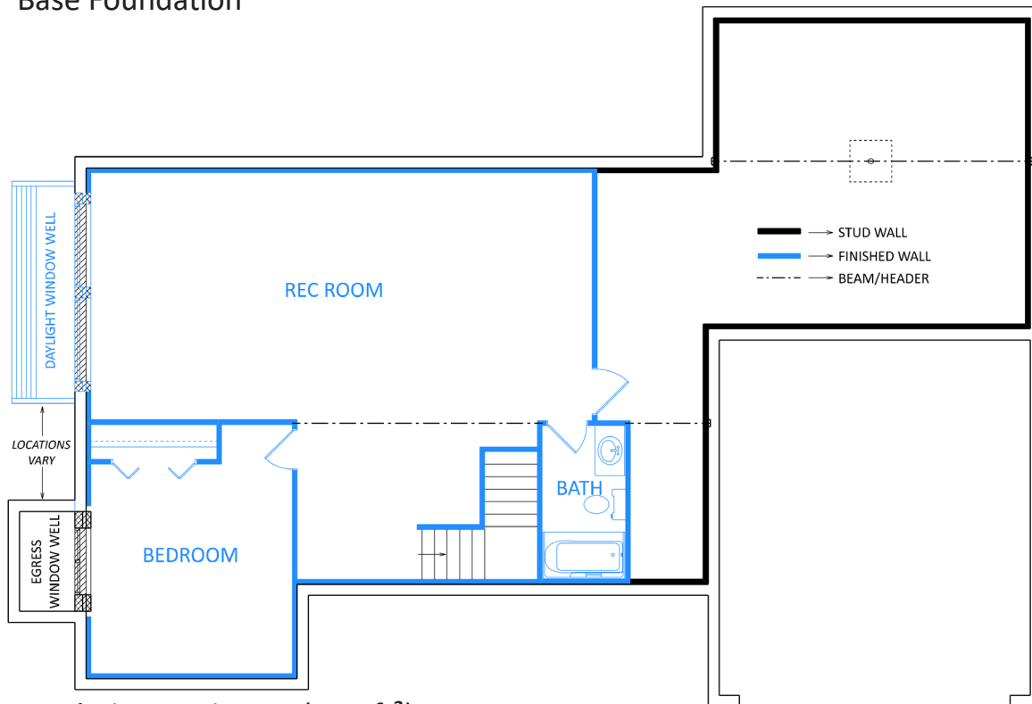
Foundation Option F1 (820 ft²)
