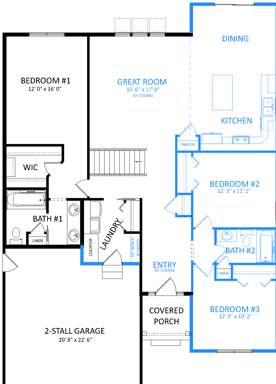
Floor Plan Option MF1 (+121 ft 2 )
