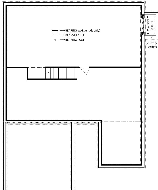
Base Foundation
