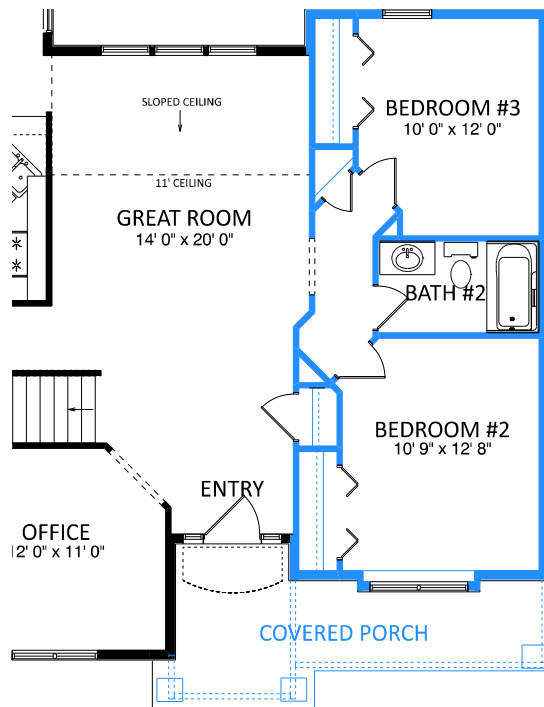
OPTION MF2 (see front elevation option FE2)
