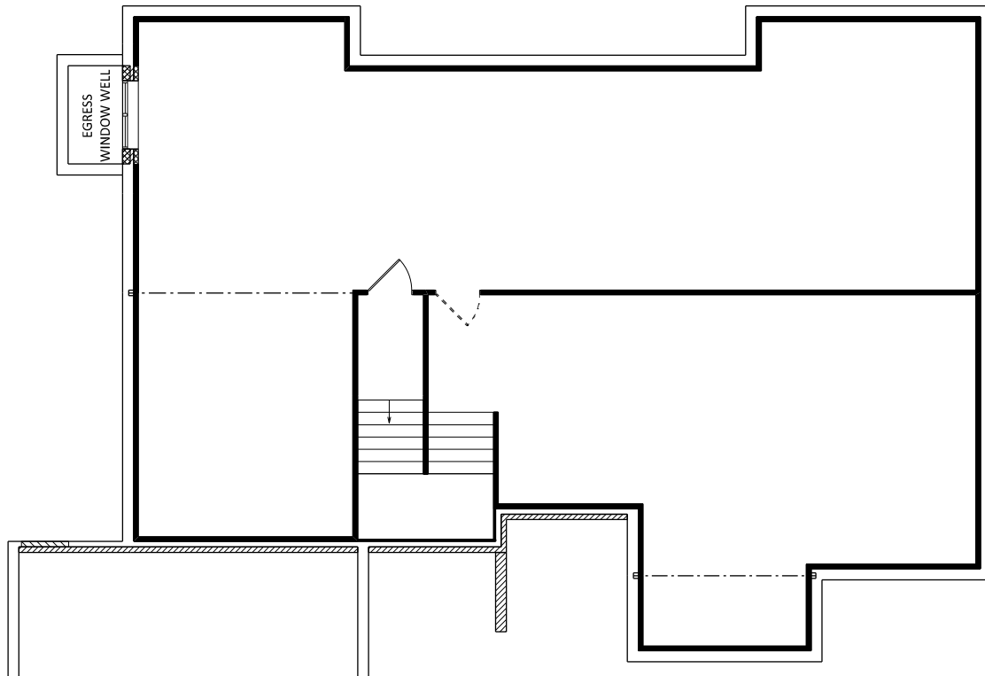
Base Foundation
