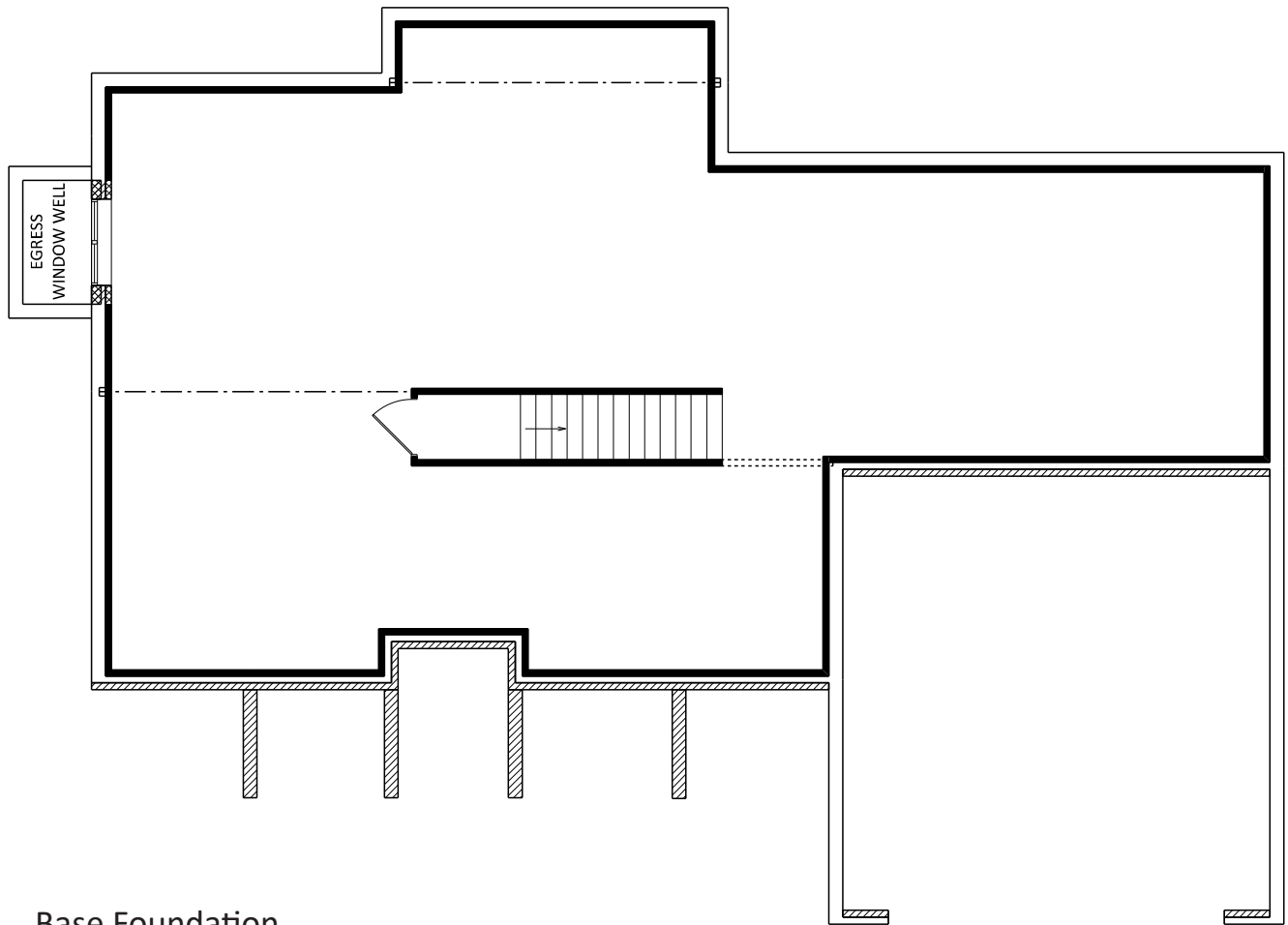
Base Foundation
